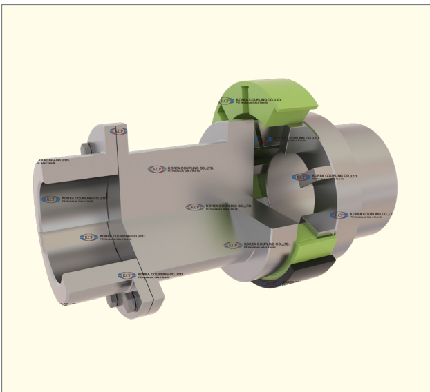
KW35 Type (Half Spacer)
